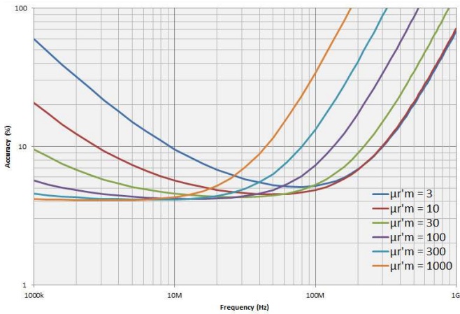
Figure 46. Permeability accuracy \left(\frac{\Delta\mu'_r}{\mu'_r}\right) vs. frequency (at F = 3 mm, typical)
