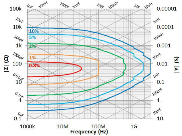
Figure 3. |Z| , |Y| Measurement accuracy when open/short/load calibration is performed. Oscillator level = -33 dBm. Point averaging factor \geq 8 within \pm 5^\circ\text{C} from the calibration temperature.
