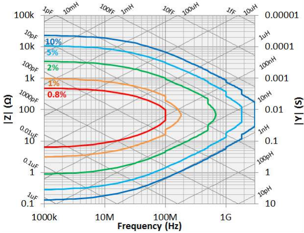
Figure 2. |Z| , |Y| Measurement accuracy when open/short/load calibration is performed. Oscillator level -13 dBm, -3 dBm. Point averaging factor \leq 7 within \pm 5^\circ\text{C} from the calibration temperature.
