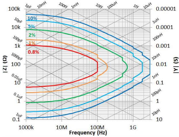
Figure 1. |Z| , |Y| Measurement accuracy when open/short/load calibration is performed. Oscillator level = -13 dBm, -3 dBm. Point averaging factor \geq 8 within \pm 5^\circ\text{C} from the calibration temperature.
