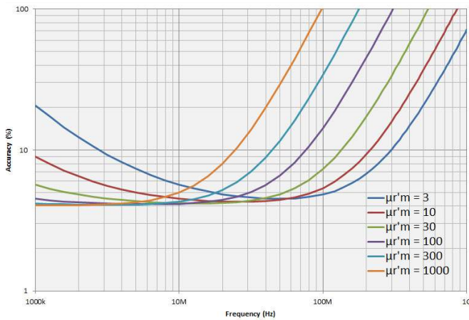
Figure 47. Permeability accuracy \left(\frac{\Delta\mu'_r}{\mu'_r}\right) vs. frequency (at F = 10 mm, typical)
