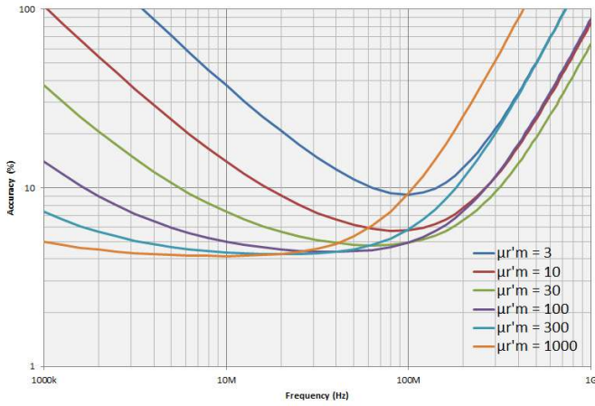
Figure 45. Permeability accuracy \left(\frac{\Delta\mu'_r}{\mu'_r}\right) vs. frequency (at F = 0.5 mm, typical)
